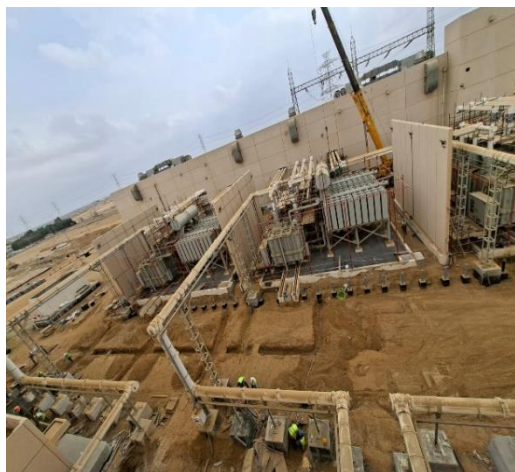
Transformer earthing system installation
