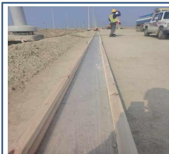
Preparation and pouring of lean concrete for Cub Stones
