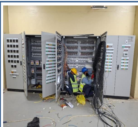
Termination of DDC/HVAC panels
